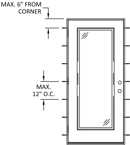
ANCHOR LAYOUT
