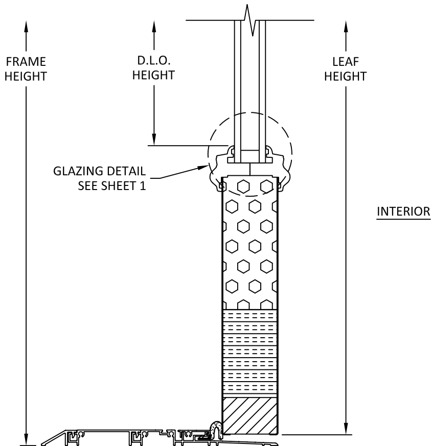
C 3 VERTICAL SECTION DOOR SILL W/ FLAT THRESHOLD NO WATER RATED
