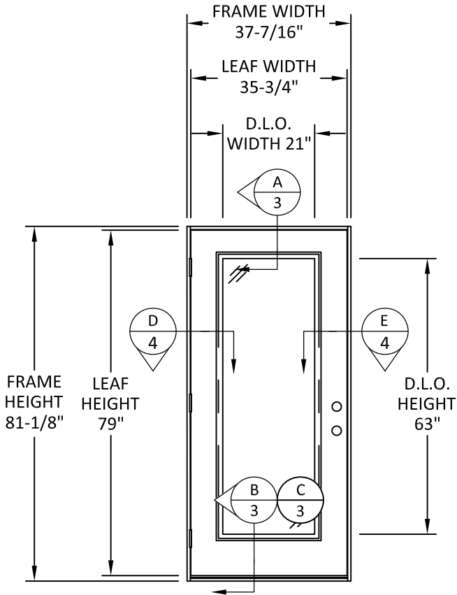
TYPICAL ELEVATION
